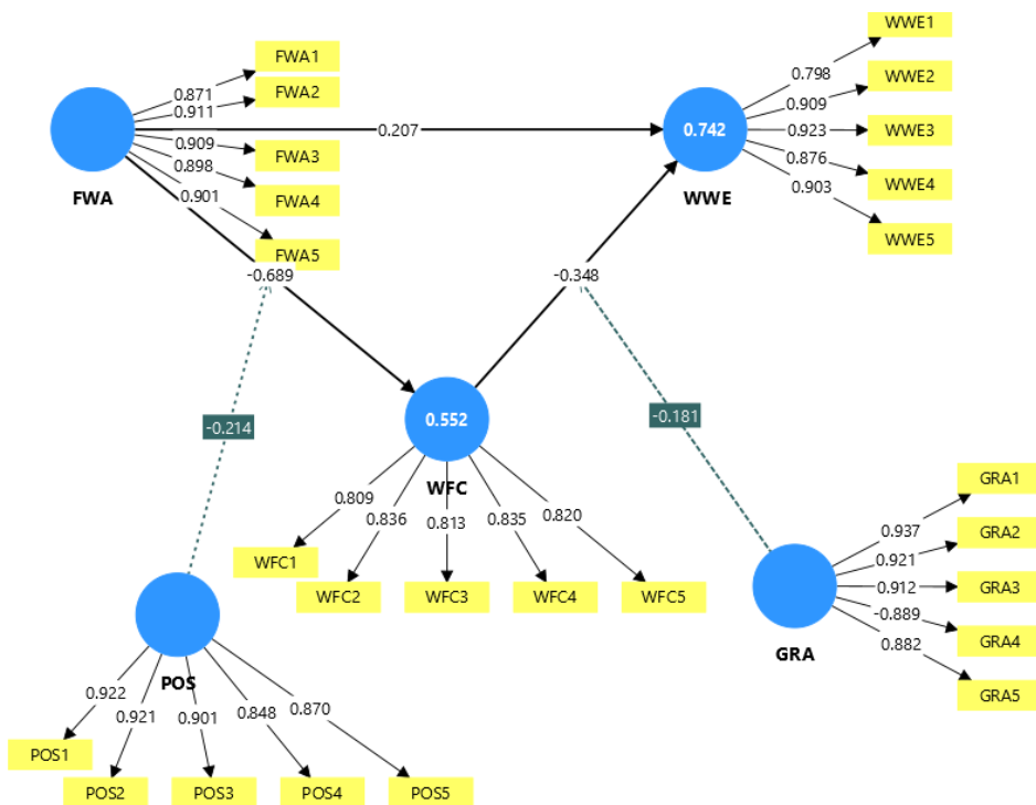
Figure 2: Measurement Model
